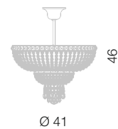
Beethoven sospensione Ø 40 cm Ø 41 cm - H 46 cm 4 x E14 40W
