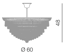
New Orleans sospensione Ø 60 cm Ø 60 cm - H 48 cm 8 x E14 40W
