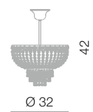
Amsterdam sospensione Ø 30 cm Ø 32 cm - H 42 cm 3 x E14 40W
